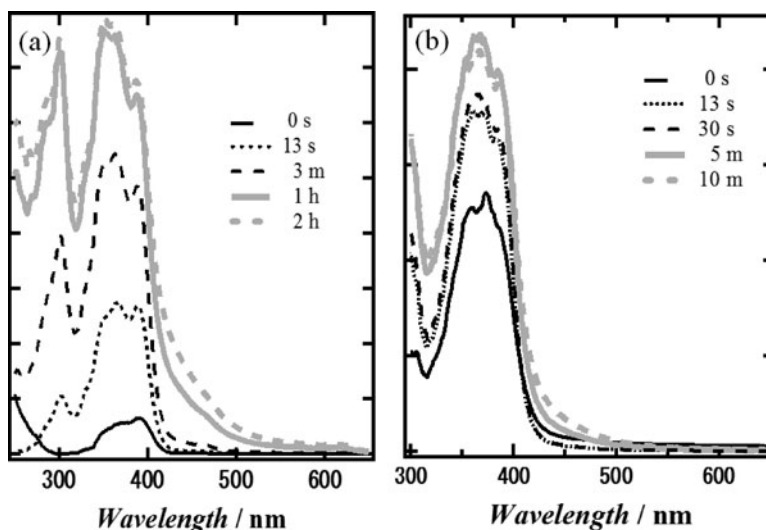
Figure 1. Change in UV-visible diffuse reflectance spectra of (a) 5 and (b) 6 depending on irradiation time of UV at 365 nm.
