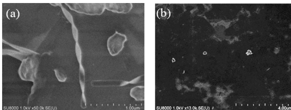
Figure 2. SEM images of nanoaggregates of (a) 5 and (b) 6 prepared at 60°C.
