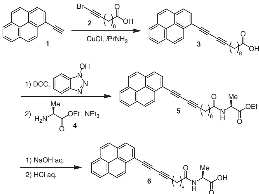
Scheme 1. Synthesis of L-alanine derivatives with a (1-pyrenyl)butadiynyl group.
